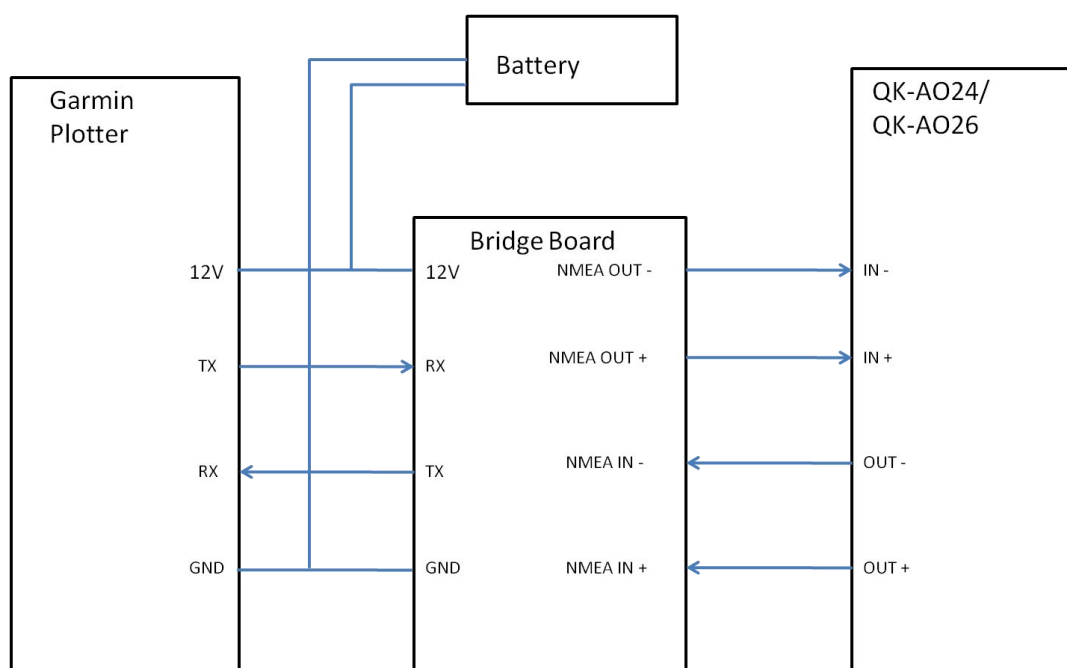
Figure 1 System connection
