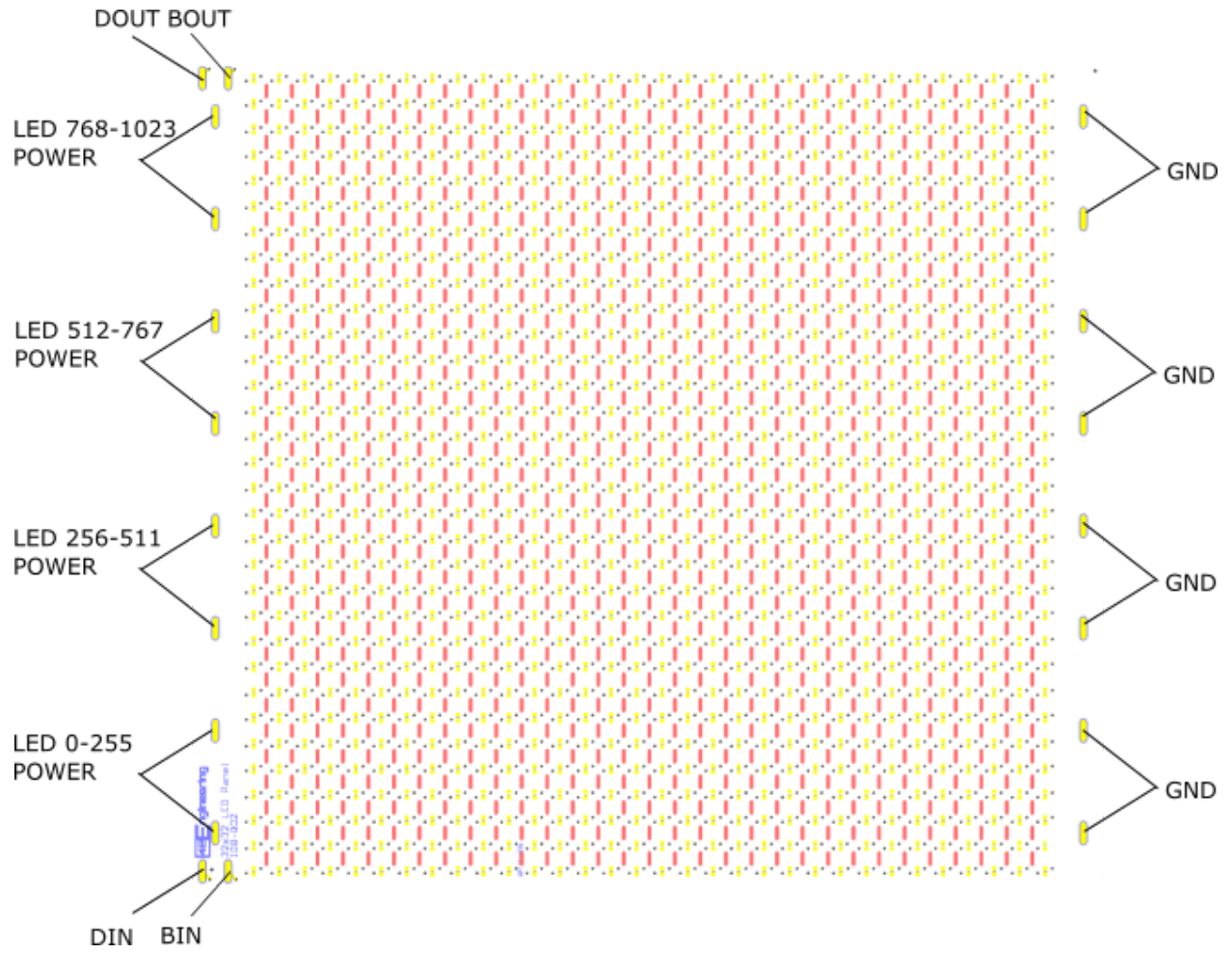
PINOUT DIAGRAM
