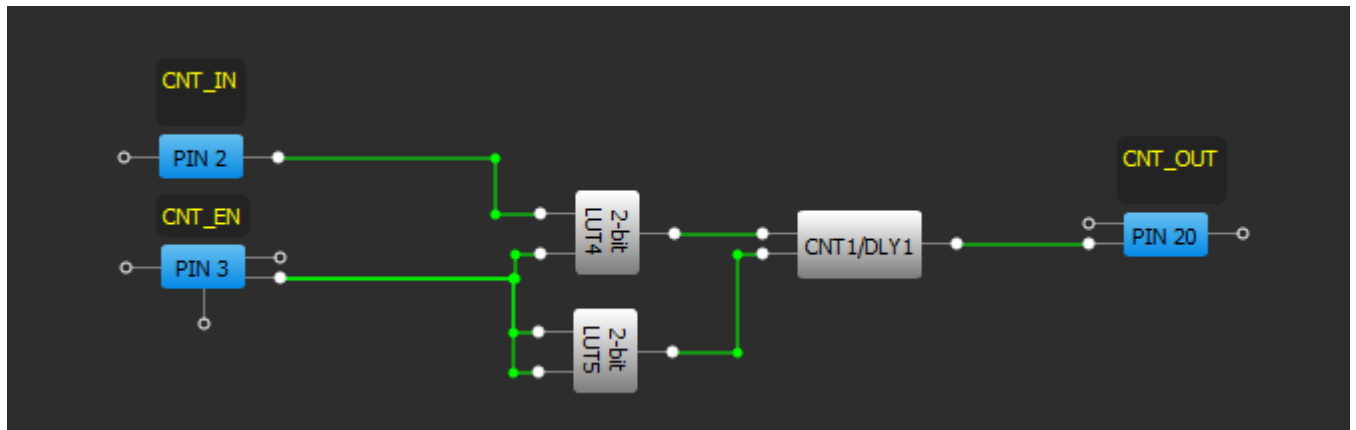
Figure 4-5. GreenPAK3 Designer
