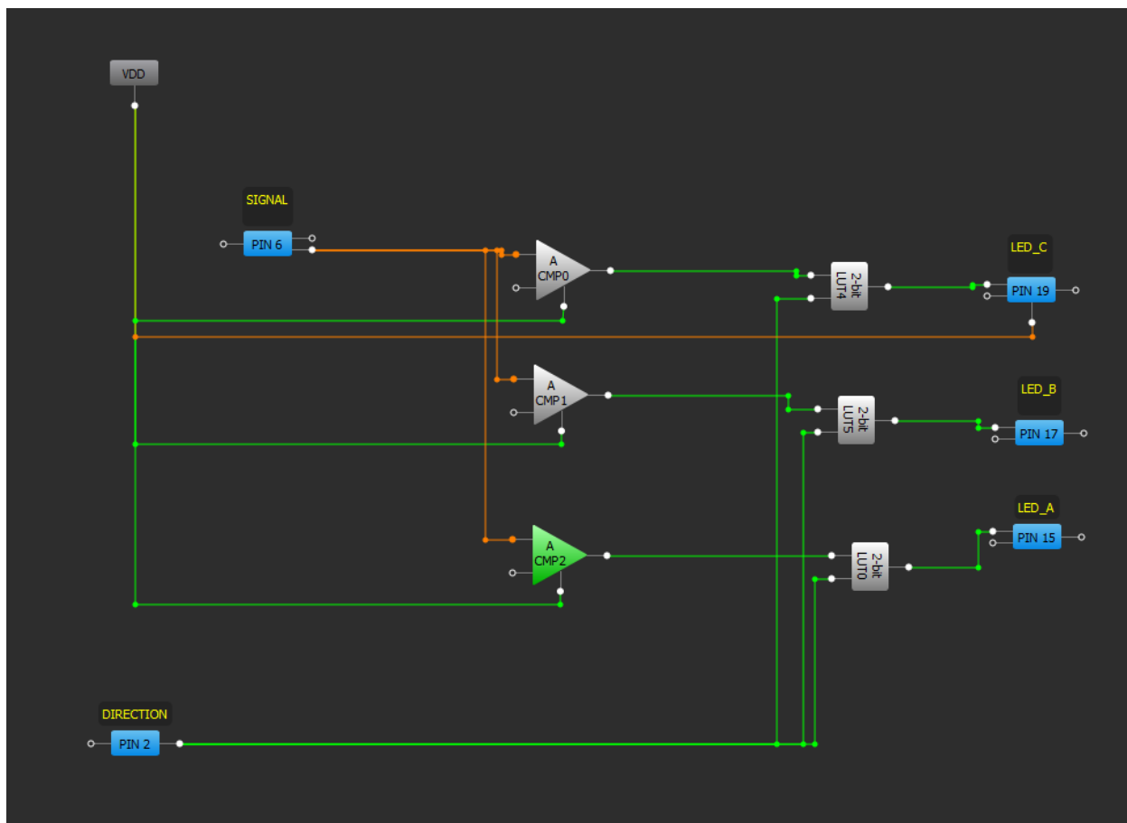
Figure 4-21. GreenPAK3 Designer
