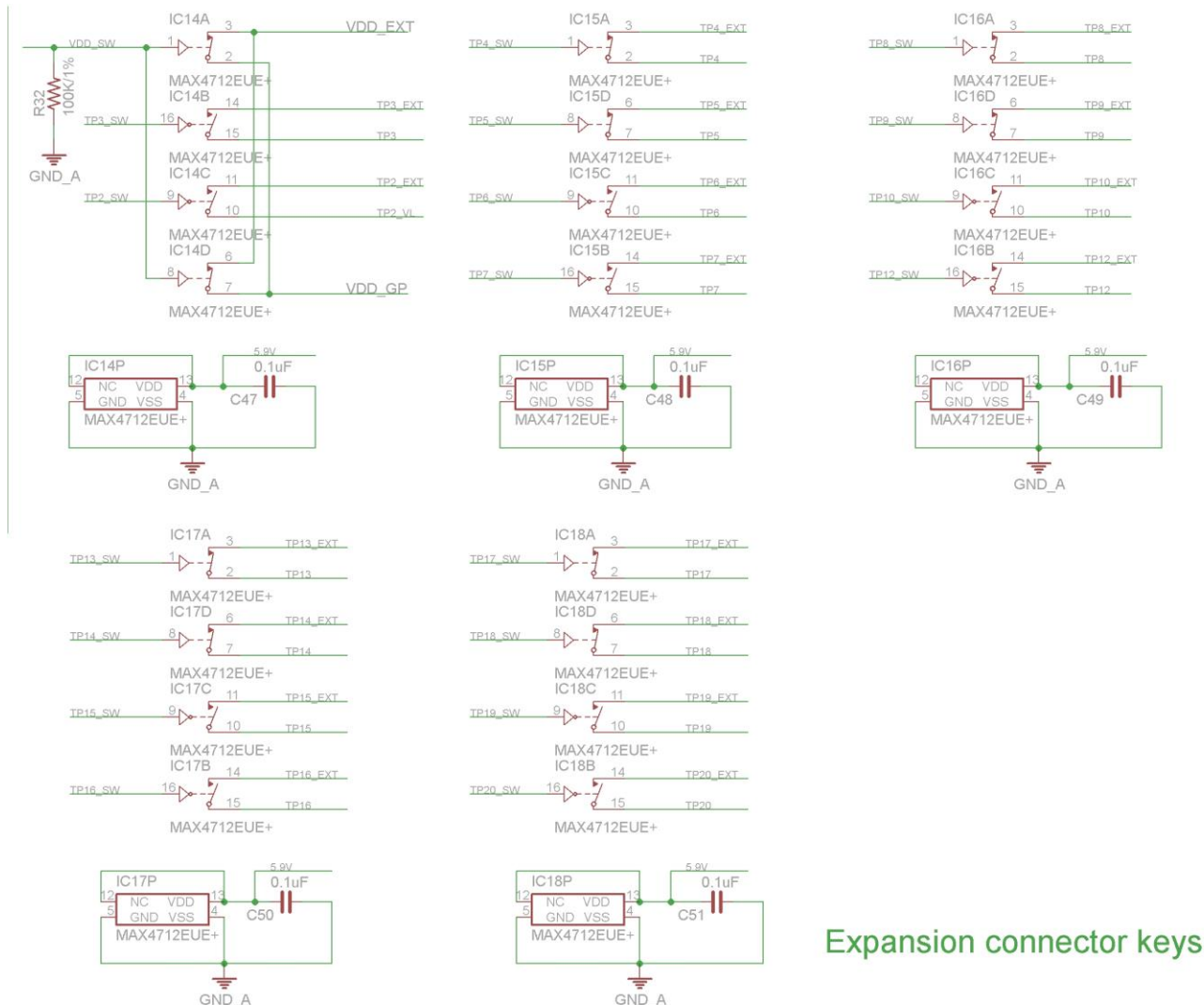
Figure 3-7. Socket and expansion connector schematic
