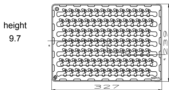
PET tray dimension
