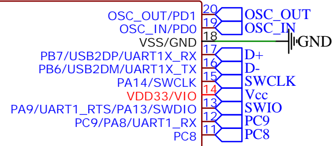
U1 CH32V305FBP6
