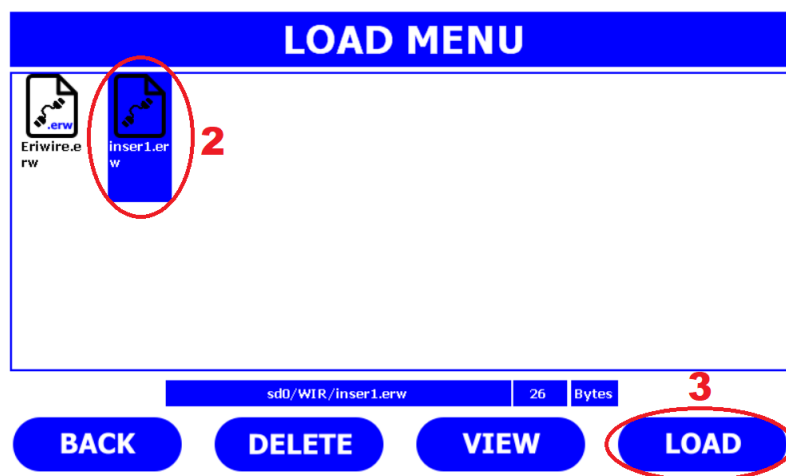
Image 12. - Load menu
