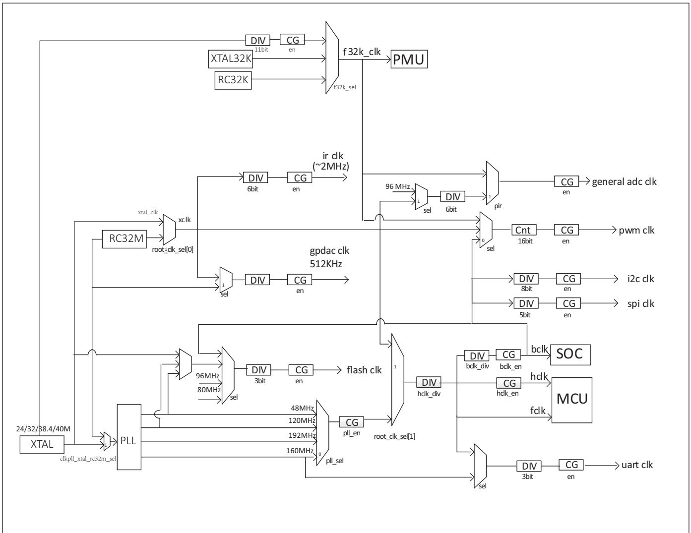
Figure 2.2: Clock Architecture
