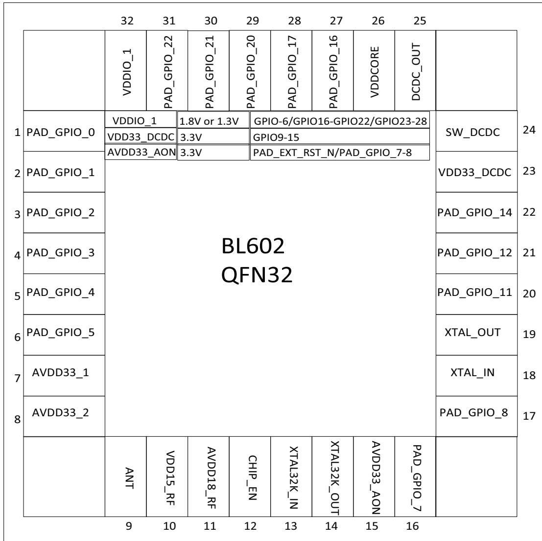
Figure 3.1: Pin layout (QFN32)
