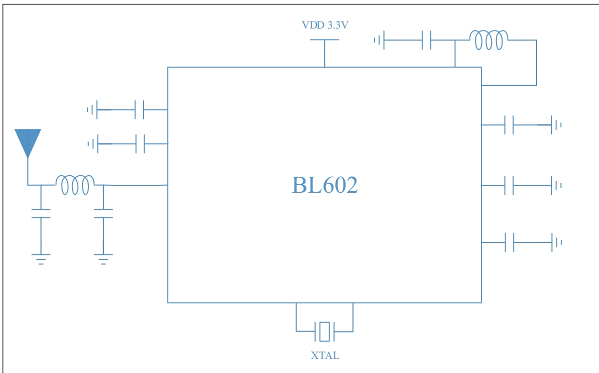
Figure 8.1: Reference Design
