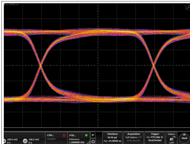
T_A = 25^\circ\text{C} Bias = 1.5 V 50 \Omega Termination Figure 23. Eye Pattern: 2.4 Gbps
