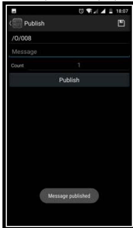
Figure 25: Message Published
