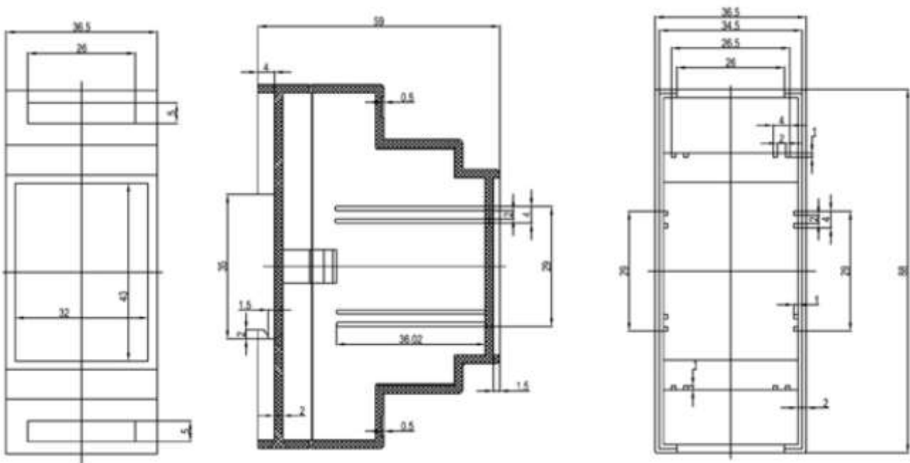
Figure 2: Box Dimensions
