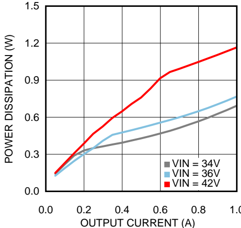
Figure 12. Power Dissipation V_{OUT} = 30\text{ V} , T_A = 25^\circ\text{C}
