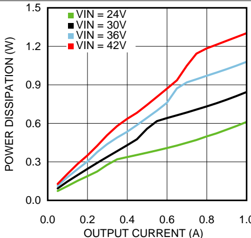
Figure 8. Power Dissipation V_{OUT} = 18\text{ V} , T_A = 25^\circ\text{C}
