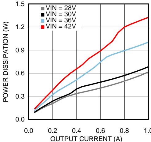
Figure 10. Power Dissipation V_{OUT} = 24\text{ V} , T_A = 25^\circ\text{C}
