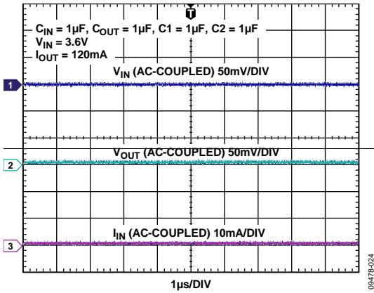
Figure 23. Typical Operating Waveforms, G = 1x
