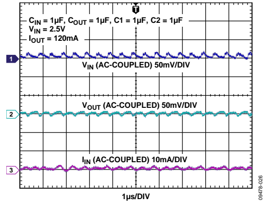
Figure 25. Typical Operating Waveforms, G = 2x
