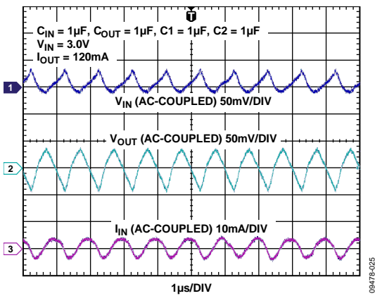
Figure 24. Typical Operating Waveforms, G = 1.5x
