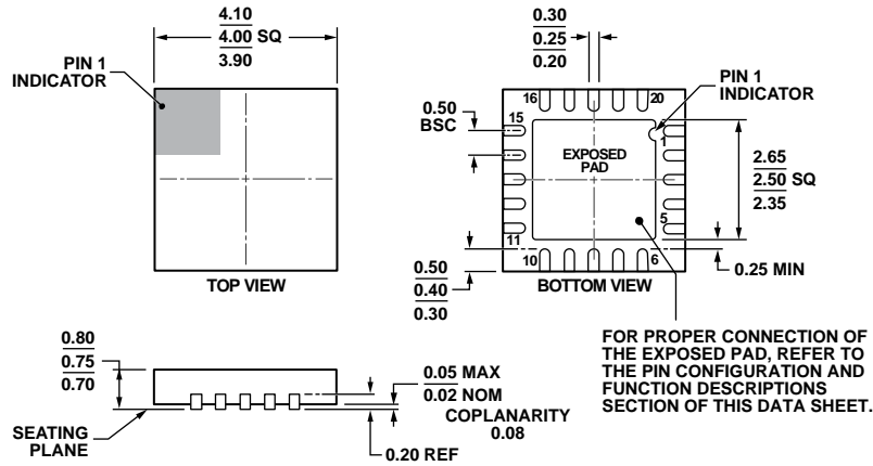
Figure 42. 20 Lead Lead Frame Chip Scale Package [LFCSP_WQ] 4 mm x 4 mm Body, Very Very Thin Quad (CP-20-10) Dimensions shown in millimeters
