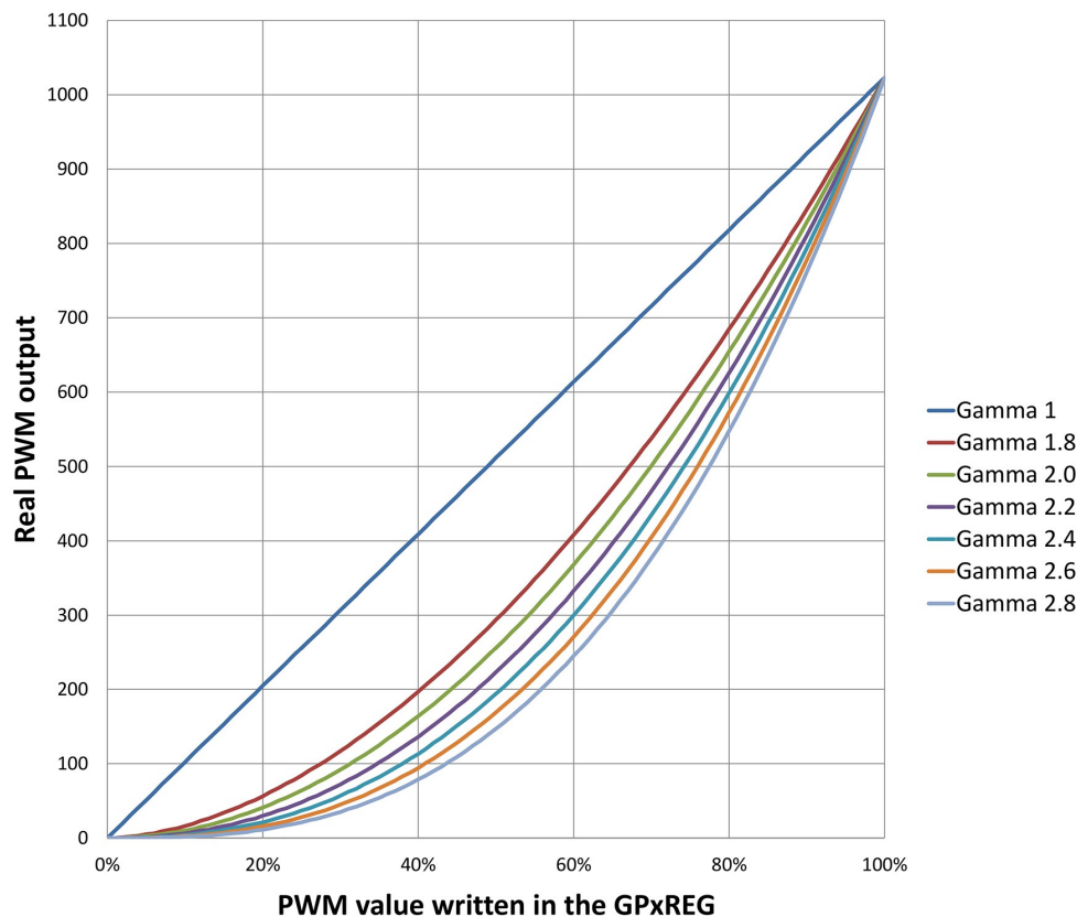
Figure 1.12: Possible gamma option
