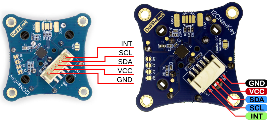
Figure 1.5: Pinout of the board in the HW V1.2
