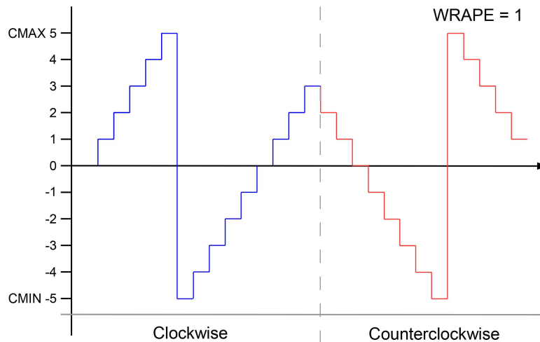
Figure 1.10: Blue and red line are the CVAL values when the encoder is rotate and the WRAPE is enabled
