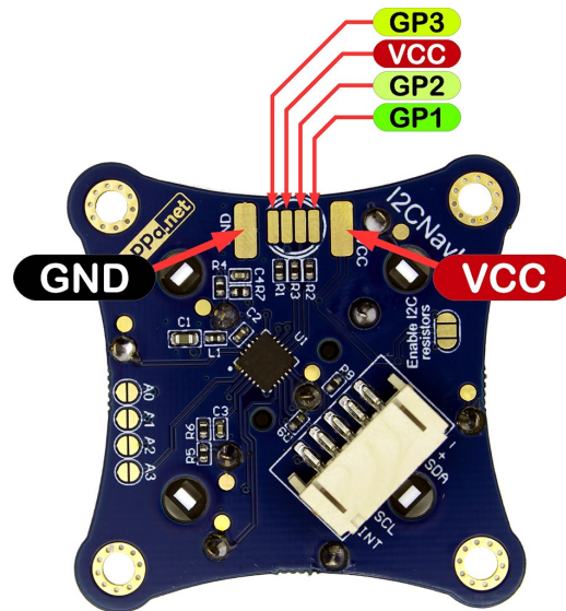
Figure 1.11: GP pins pinout
