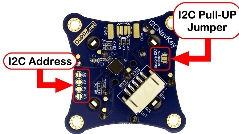
Figure 1.6: Jumper location of the pull-up resistor and of the address
