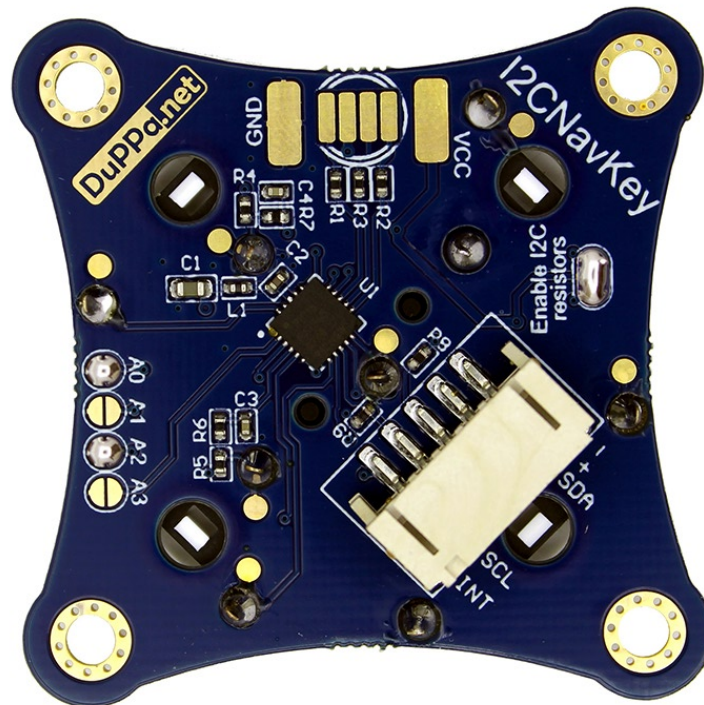
Figure 1.7: Example of jumper soldered: A0 and A2 shorted and also the SJ5 is shorted enabling the pull-up resistors
