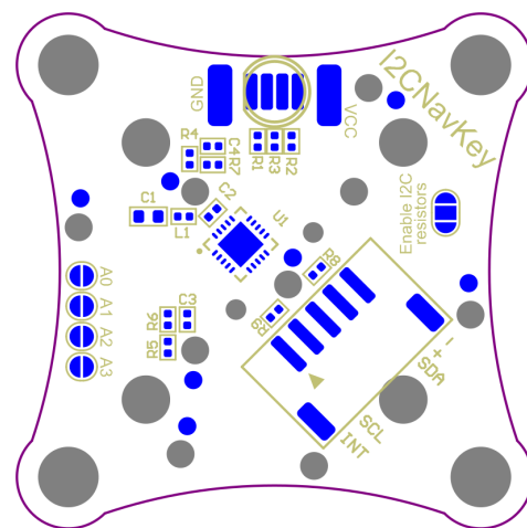
Figure 1.2: Bottom view of the board
