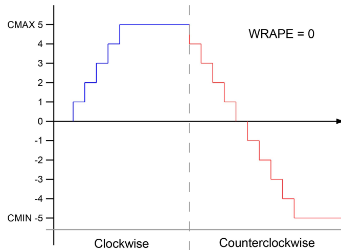
Figure 1.9: Blue and red lines are the CVAL values when the encoder is rotated and the WRAPE is disabled
