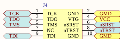
AVR JTAG 2.54mm male
