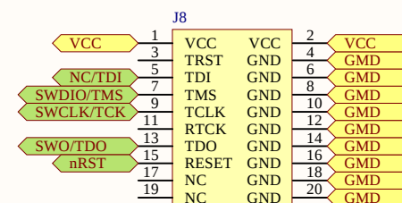
2x10 2.00mm
